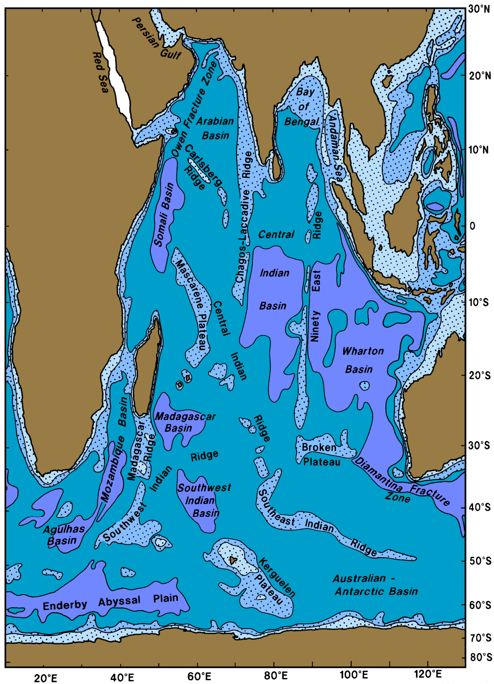
Fig. 11.1. Topography of the Indian Ocean. The 1000, 3000, and 5000 m isobaths are shown, and regions less than 3000 m deep are shaded. South of Australia the Indian Ocean extends to Tasmania (146° 55'E). See Figure 8.3 for the topography east of 125°E.
