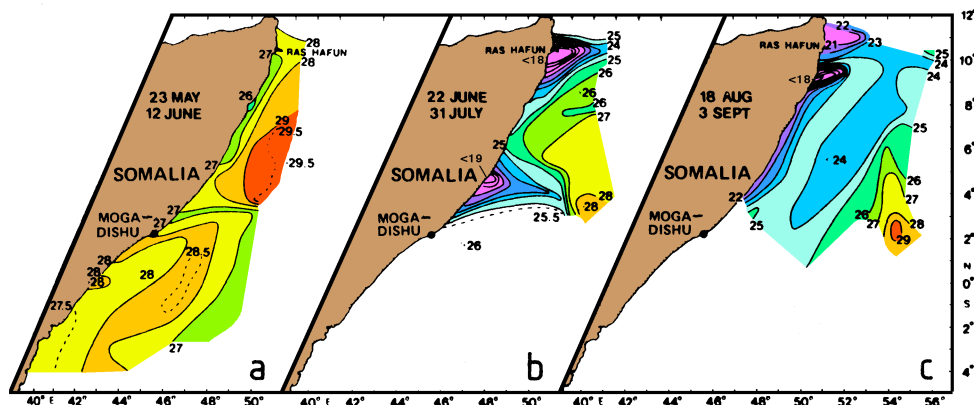
Fig. 11.16. Development of the Somali Current during the onset of the Southwest Monsoon as seen in the sea surface temperature during 1979. (a) Advection of warm water south of 3^{\circ}\text{N} and coastal upwelling north of 3^{\circ}\text{N} , (b) two gyres with upwelling regions near 4^{\circ}\text{N} (minimum temperature <19^{\circ}\text{C} ) and Ras Hafun (minimum temperature <18^{\circ}\text{C} ), (c) continuous northward flow and upwelling near Ras Hafun (minimum temperature <17^{\circ}\text{C} ). From Evans and Brown (1981).
